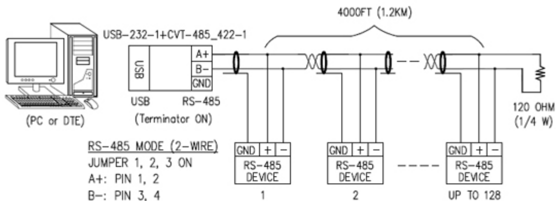
FIGURE 1: MASTER-SLAVE MULTI-DROP CONNECTIONS (RS-485)
